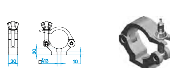
CLP-P645 Clamp slim (60-63.5 mm) SWL 510 kg (SF 8:1)
