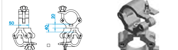
CLP-P636 weight = 1.5 kg Swivel coupler (60-63.5 mm) SWL 650 kg (SF 8:1)
