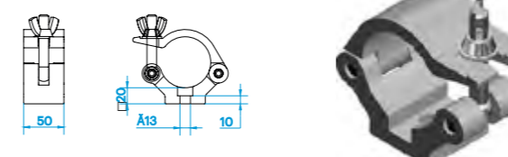
CLP-P635 weight = 0.65 kg Clamp (60 mm) SWL 650 kg (SF 8:1)
