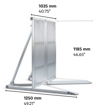
Crowd barrier – variable corner
