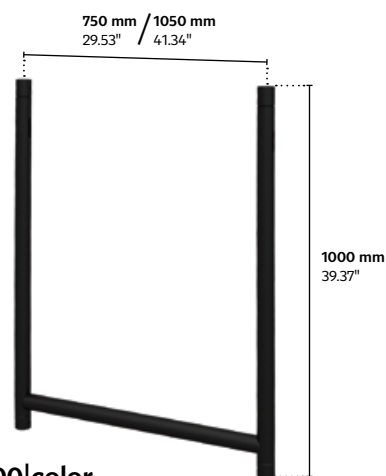
MLA-H750×1000|color MLA-H1050×1000|color
