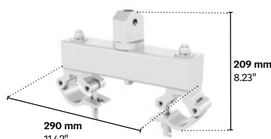
MRT1-04|StabilizerHorizontalL
