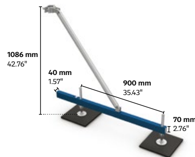
MT1-05|LongOutrigger
