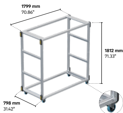
MMC-1.80x1.80x0.80 m - 100-mm wheels
