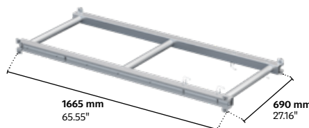
MMC-telescopic frame
