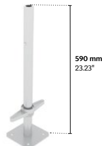
ScrewjackTR38×1-590
