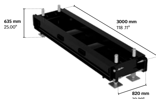
S-MT-Q-05|Outrigger3000
