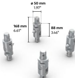
MRT1-07B|Hinges|4pcs
