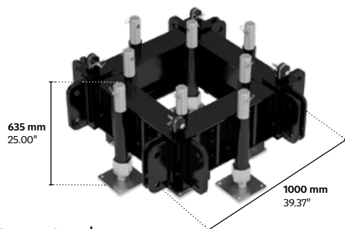
S-MT-Q-01|Base
