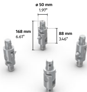
MT1-07B|SetHinge|4pcs
