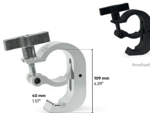
CELL601 / CELL601|Anodised
