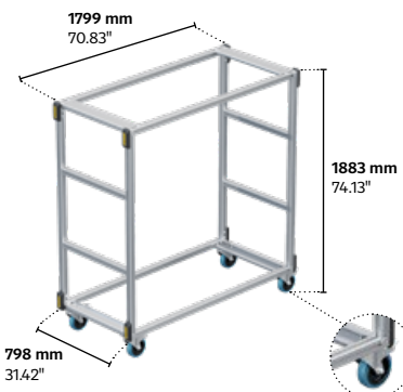
MMC-1.80x1.86x0.80 m - 160-mm outdoor wheels
