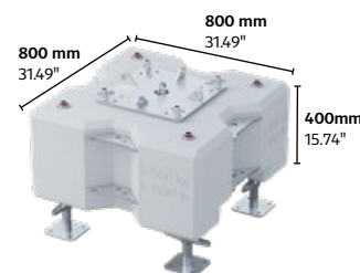
Concrete Ballast Base MCBB
