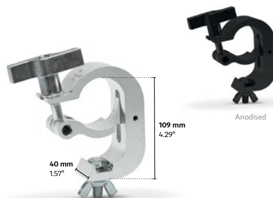
CELL602 / CELL602|Anodised
