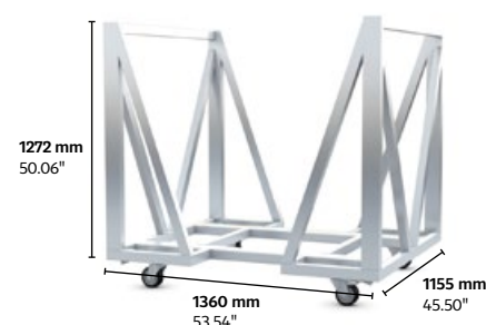
Crowd barrier – cart up to 10 barriers
