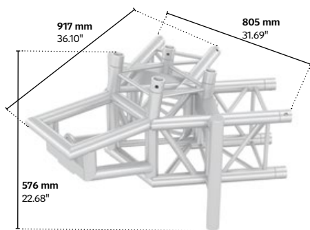
MRT1-01B|BaseCorner
