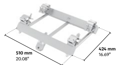
MRT1-05|StabilizerVertical
