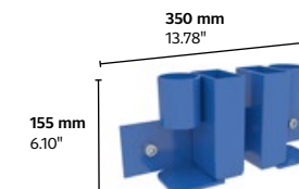
MT1-OutriggerHolder|2pcs
