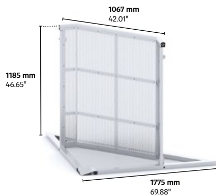
Crowd barrier – inside corner 90°
