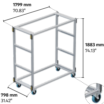
MMC-1.80×1.80×0.80 m – 160-mm outdoor wheels
