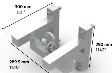
MT1-09|BracketForMotor|Sleeve
