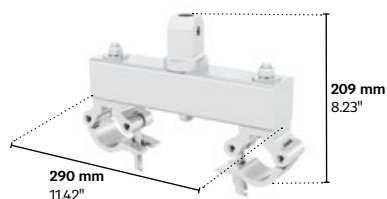
MRT1-04|StabilizerHorizontalR
