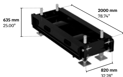
S-MT-Q-05|Outrigger2000
