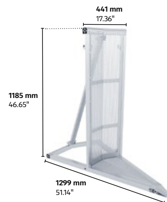
Crowd barrier – inside corner 30°
