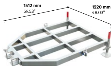
MT1-01|BallastBase
