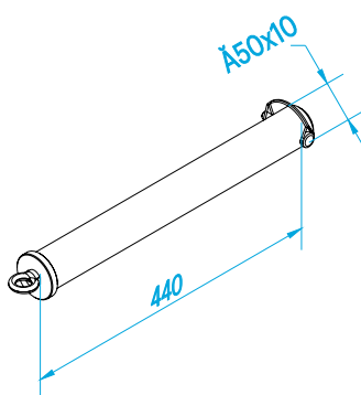
Dead hang Pin
