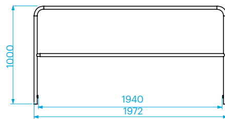
EasyRail railing. SM-RAIL-L200.
