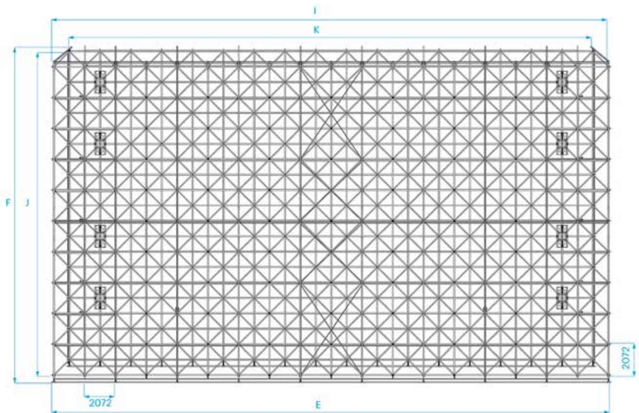
Top view
