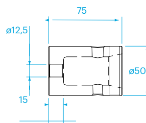
CCS6-651 weight = 0,280 kg Female conical coupler With 12,5 mm hole for bolts M12
