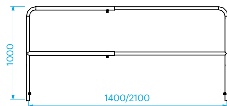
EasyRail railing. SM-RAIL-L140/210.
