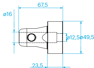
CCS6-652-23,5 weight = 0,469 kg Half conical coupler Offset 23,5 mm, 12,5 mm hole To be used with a M12 Hexagon head
