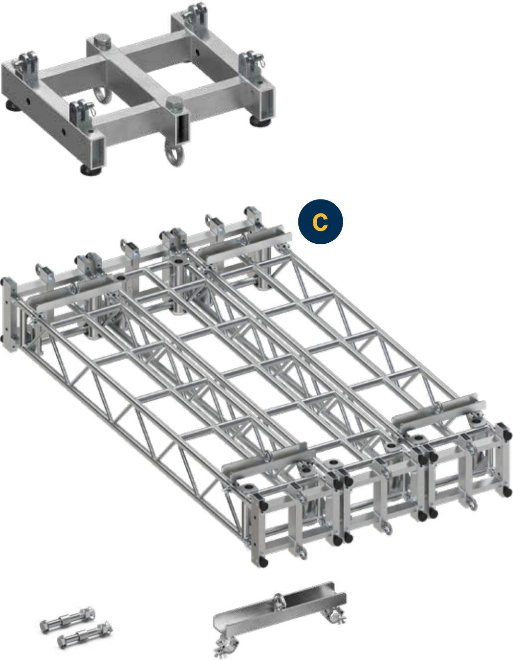
KIT-65 Screws for coupling the trusses together.
